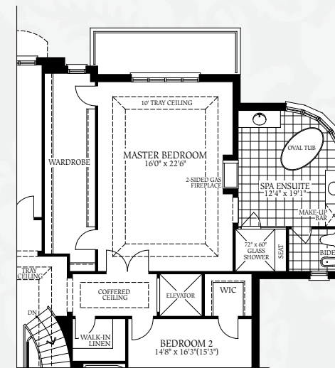
SECOND FLOOR WITH OPTIONAL ELEVATOR
