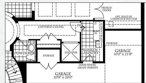
FIRST FLOOR WITH OPTIONAL ELEVATOR
