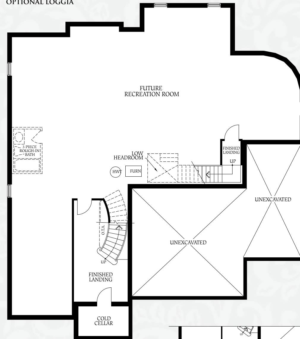
BASEMENT PLAN ELEVATION A
