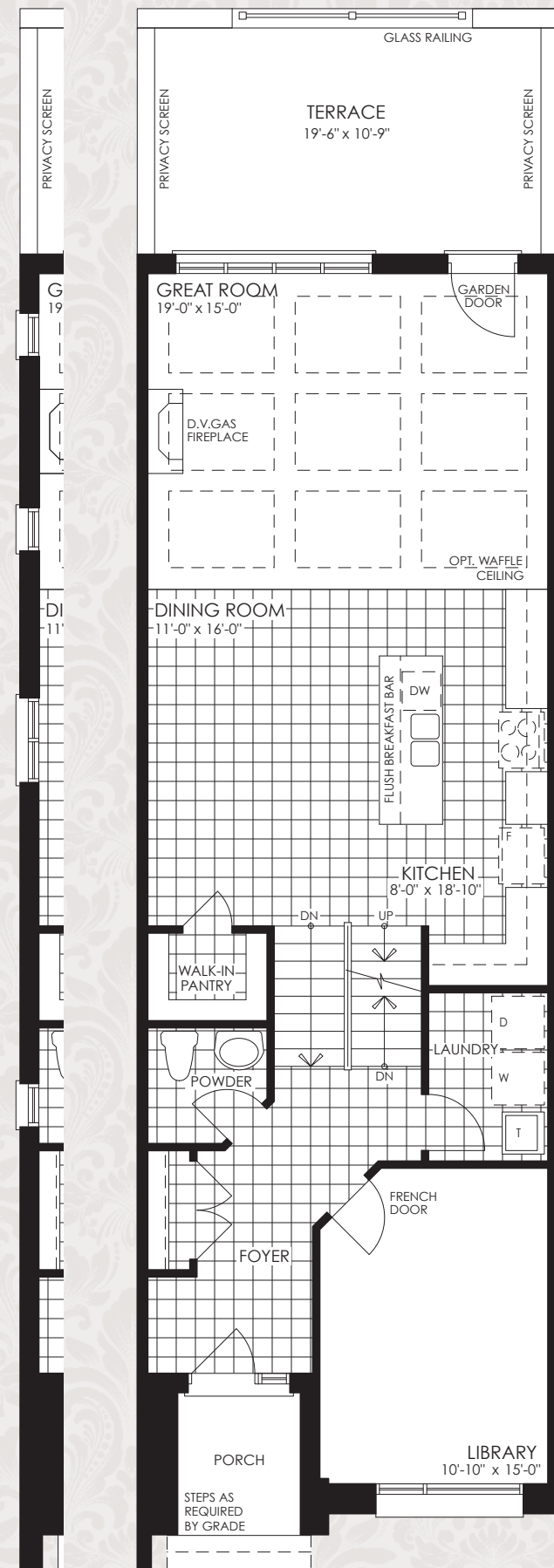
Main Floor End Unit
