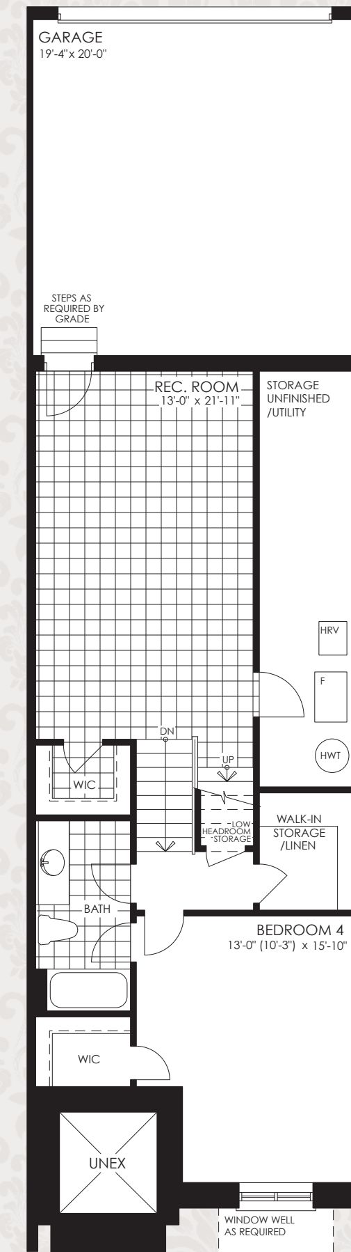
Optional Finished Lower Floor
